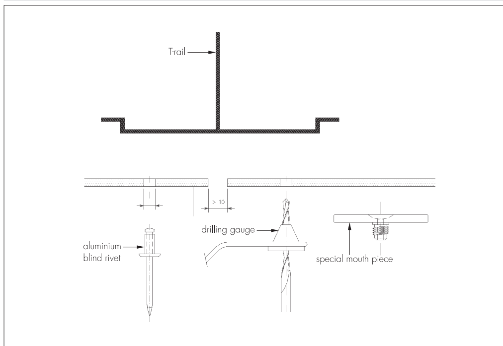
Figure 2 Typical installation detail
