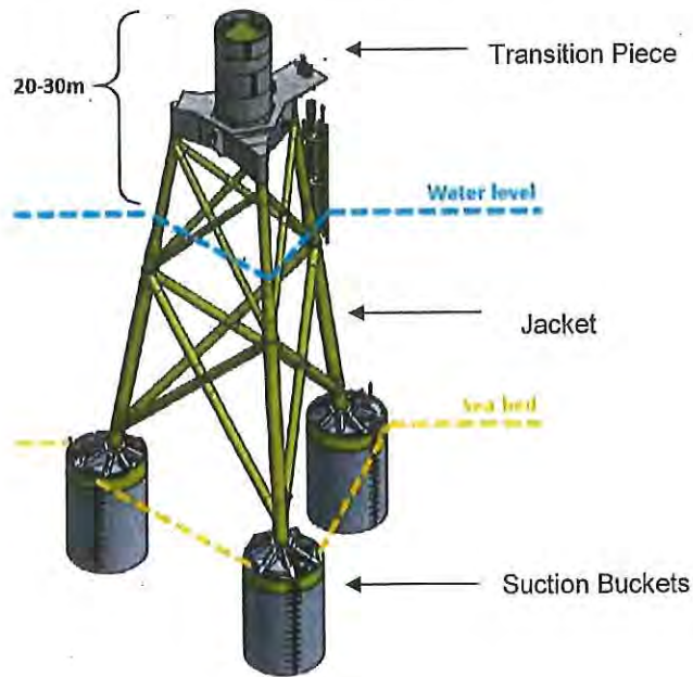
Figure 1. Schematic of foundations (incl. jacket) to be installed
