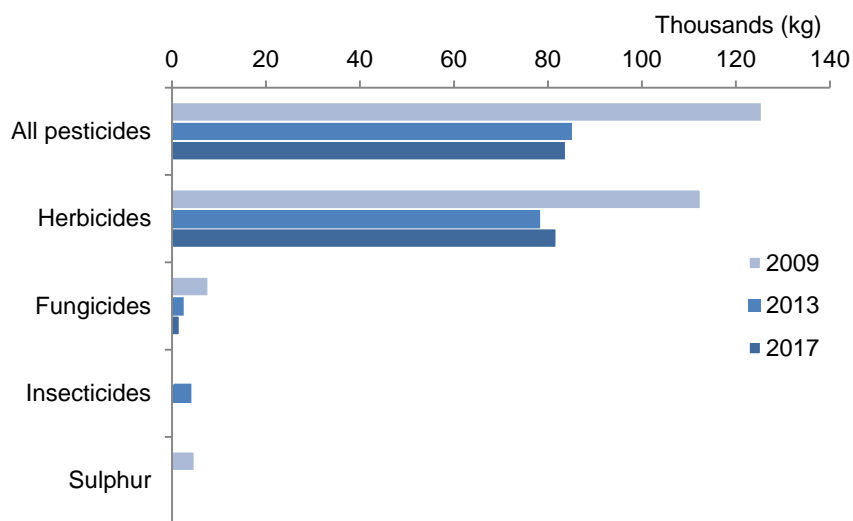
Figure 8 Weight of major pesticide groups applied to grass crops in Scotland 2009-2017
